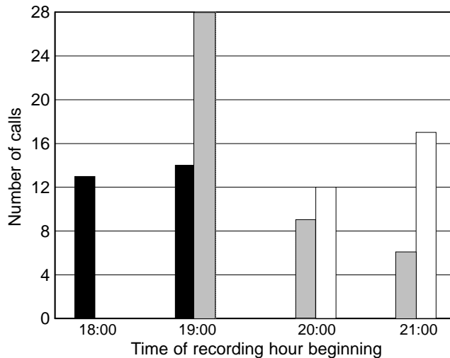
FIG. 3. Frequency distribution of P. macrotis echolocation calls of different durations recorded for the 60 min period beginning at 18:00 h, 19:00 h, 20:00 h, and 21:00 h. Calls \leq 5 ms long are shown by solid black bars, 6–10 ms long calls as gray bars, and calls \geq 11 ms as open bars
